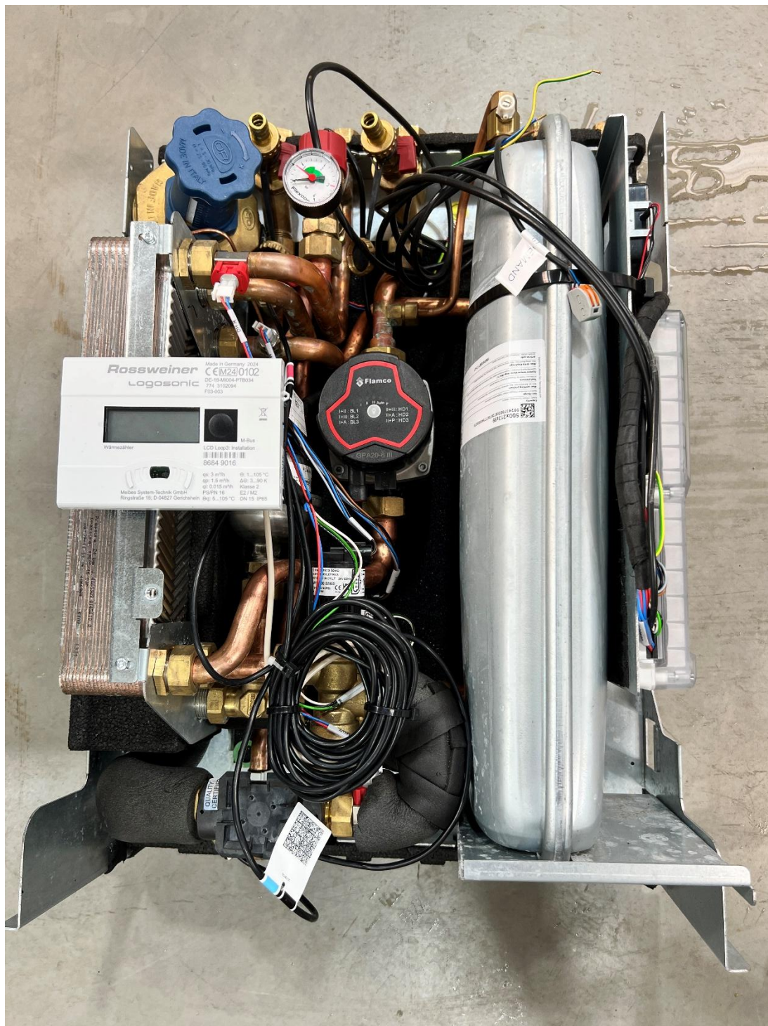
Figure 21 - HIU with Outer Case Removed
