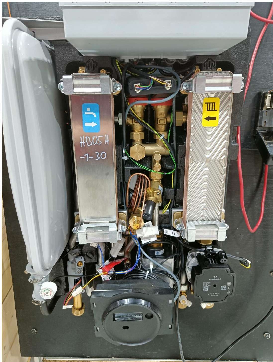
Figure 21 - HIU with Outer Case Removed
