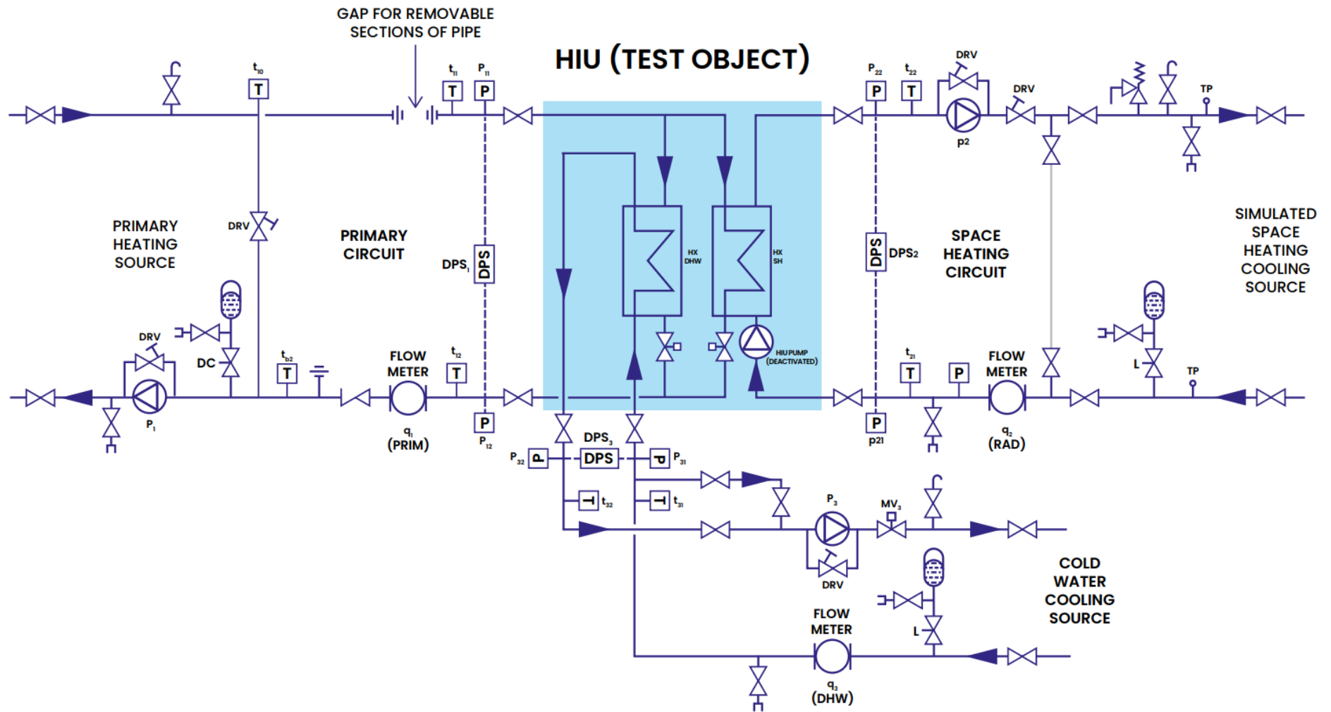
Figure 1 - EIL's HIU Test Rig Schematic which is taken from Appendix B, Figure 4, of Technical Standard for UK HIU Test Regime V3-Rev002: March 2026
