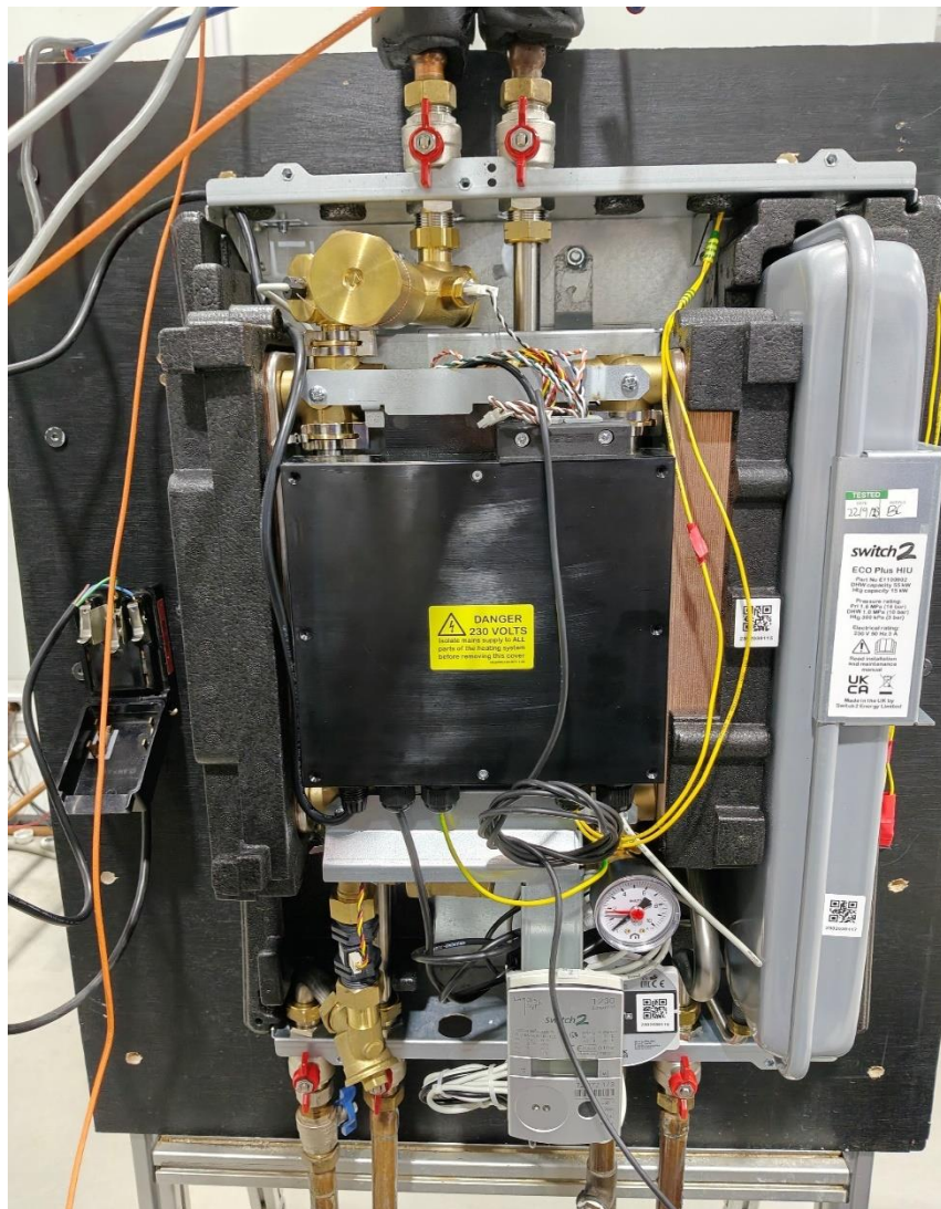
Figure 21 - HIU with outer case removed
