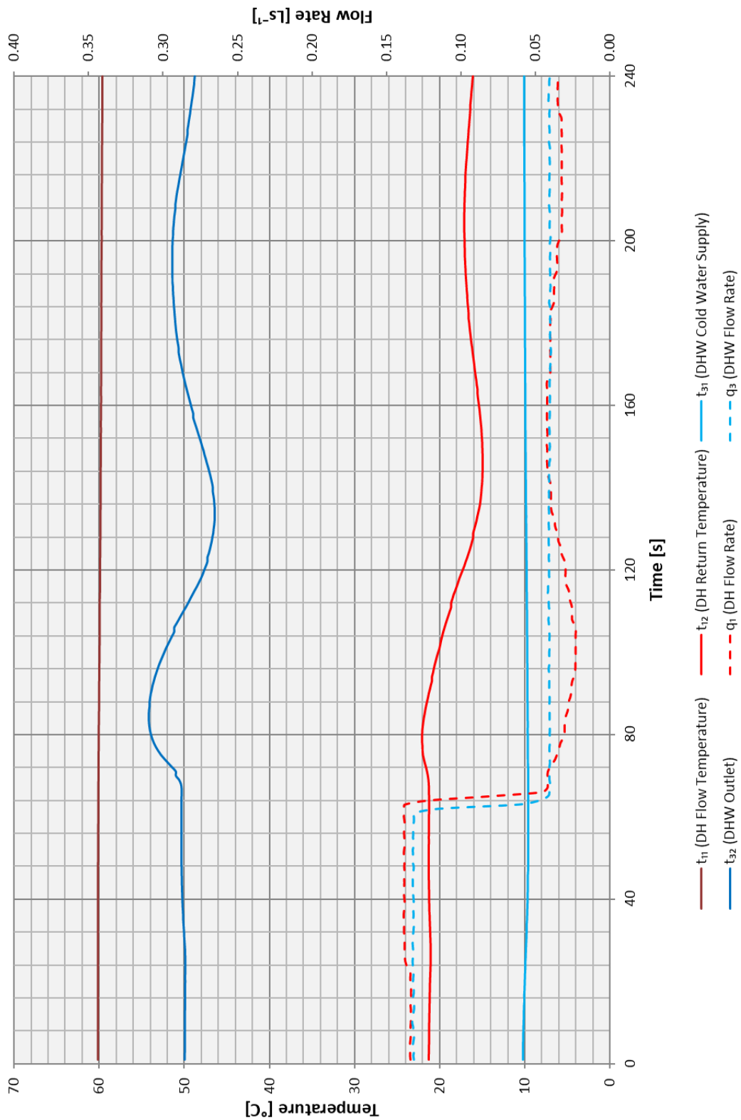
Figure 7.10 - Test 3d – Low Flow DHW at 60 °C
